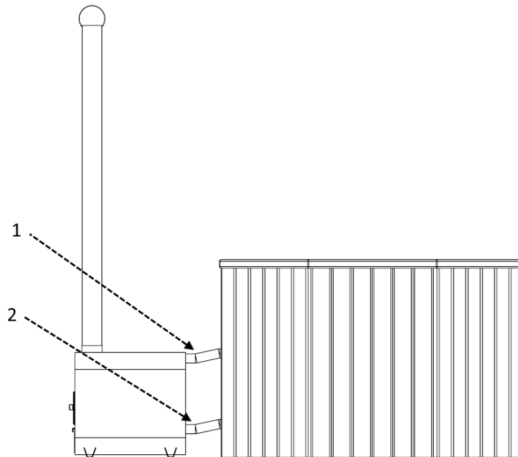
Image 6. Locations of the hose clamps of the external heater
