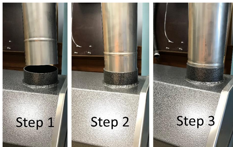
Image 9. Chimney assembly
